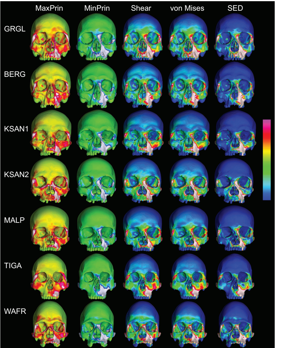
Figure 7 Strain distributions in the ALL-HUM models: P 3 biting. Color maps of strain distributions in the ALL-HUM variants of “extreme” and “average” modern human cranial FEMs during premolar (P 3 ) biting. Scales are set to range from −150–150 \mu\epsilon for both maximum principal strain (MaxPrin) and minimum principal strain (MinPrin), from 0–300 \mu\epsilon for both maximum shear strain (Shear) and von Mises strain (von Mises), and from 0–0.5 J/mm 3 for SED. White regions exceed scale. Models are shown at the same height.
