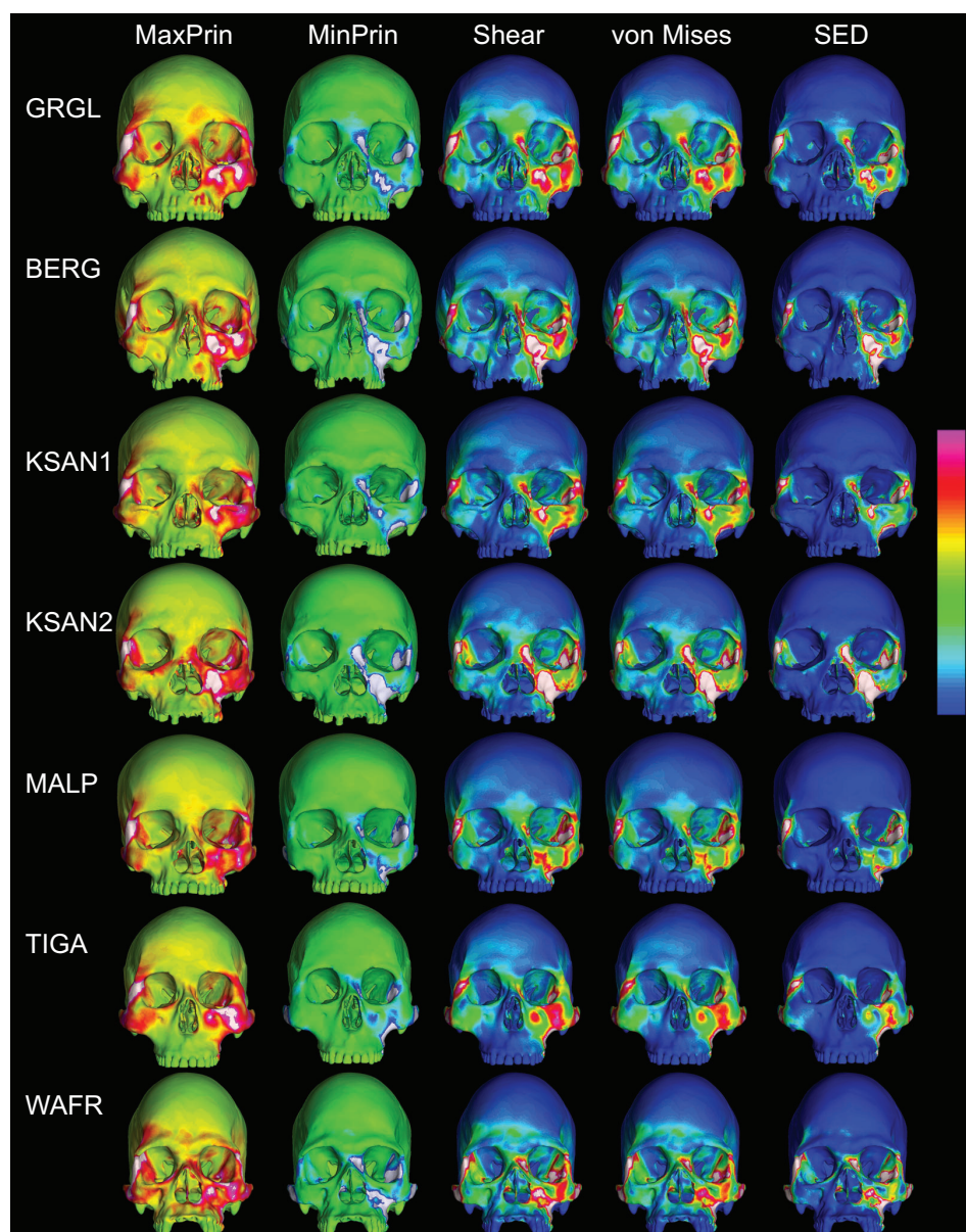
Figure 8 Strain distributions in the ALL-HUM models: M^2 biting. Color maps of strain distributions in the ALL-HUM variants of “extreme” and “average” modern human cranial FEMs during molar ( M^2 ) biting. Scales are set to range from -150 – 150 \mu\epsilon for both maximum principal strain (MaxPrin) and minimum principal strain (MinPrin), from 0 – 300 \mu\epsilon for both maximum shear strain (Shear) and von Mises strain (von Mises), and from 0 – 0.5 \text{ J/mm}^3 for SED. White regions exceed scale. Models are shown at the same height.
